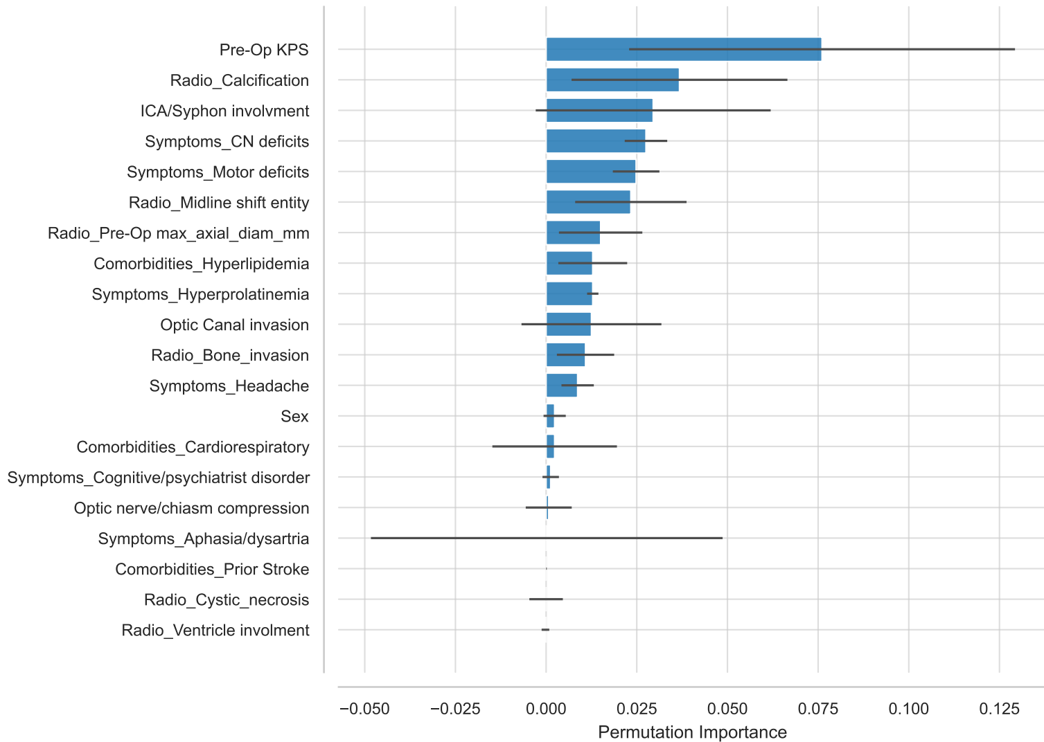
Feature Importance (LR)
